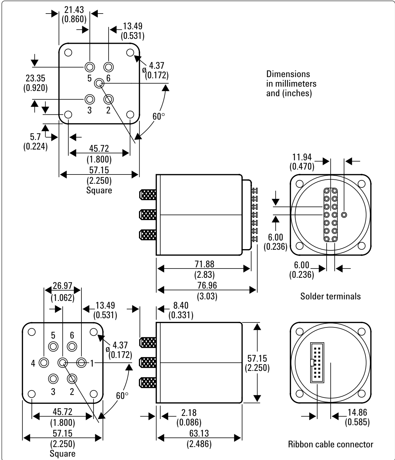
Figure 6. Product outline
